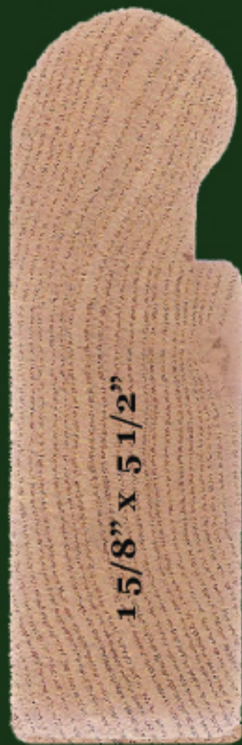
Handrail 640
