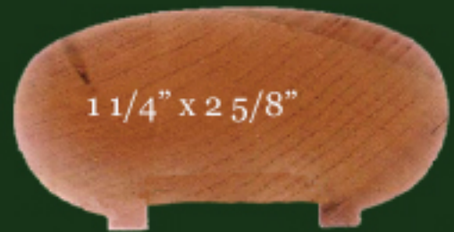
Handrail 618
